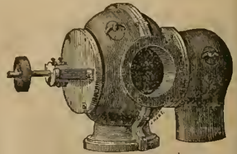
HORIZONTAL FLUME, Patented April 1st, 1873.
