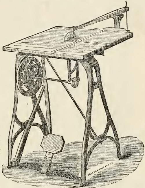
COMBINED SCROLL AND CIRCULAR SAW, $40.
